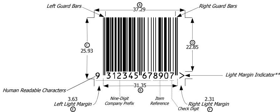
Nominal size (Magnification 100%) EAN-13 bar code symbol illustration
